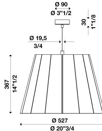
Technical drawing Size ref. image mm - inch
